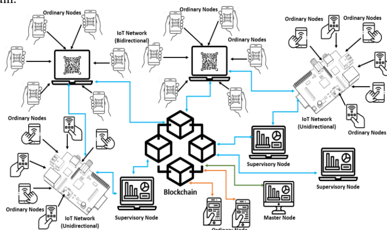
Figure 1. System Architecture
