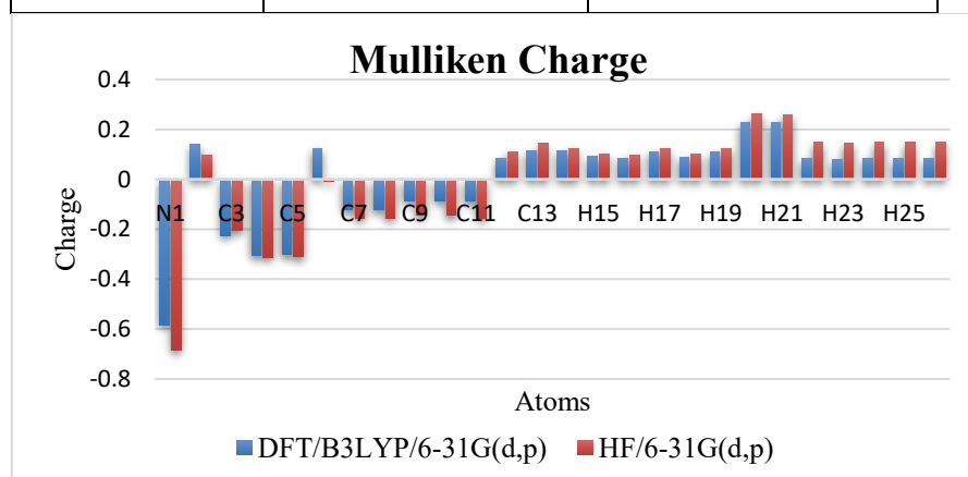
Fig.6. Mulliken's atomic charges of 2-methyl-1-phenylpropan-2-amine
