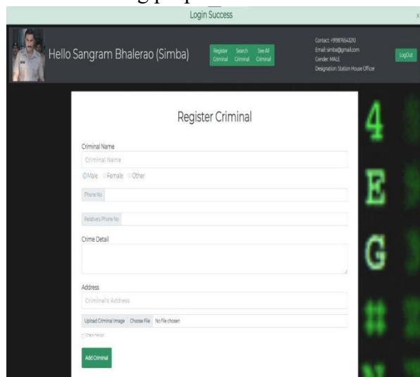
Fig.2: Registration Module
