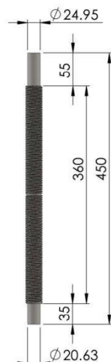
Figure 1: The Power screw
