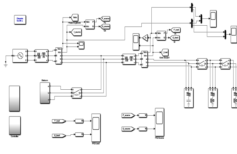
Figure 3. Simulation model of Three Phase System Traditional STATCOM
