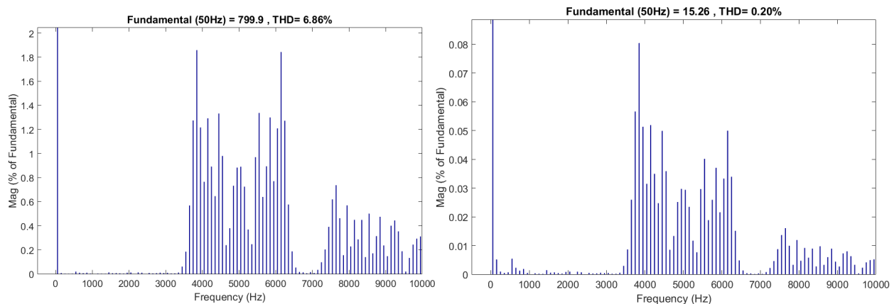
Fig 7. Output voltage and current THD of 17 level inverter with APD-PWM and modulation index is 1
