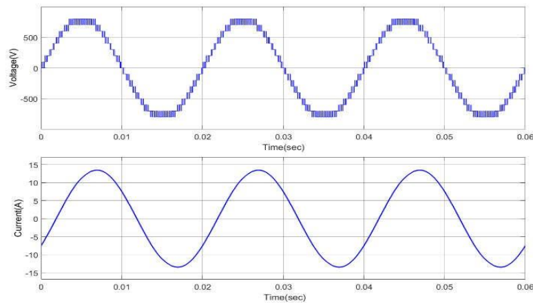
Fig 2. 17 level output voltage and load current with LS-PWM when modulation index is 1 and load is 50\Omega and 50\text{mH}
