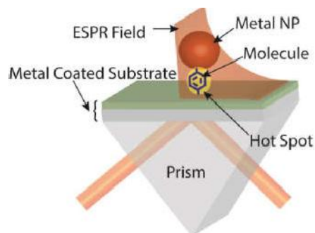
Fig.7. ESP-LSP coupled biosensor
