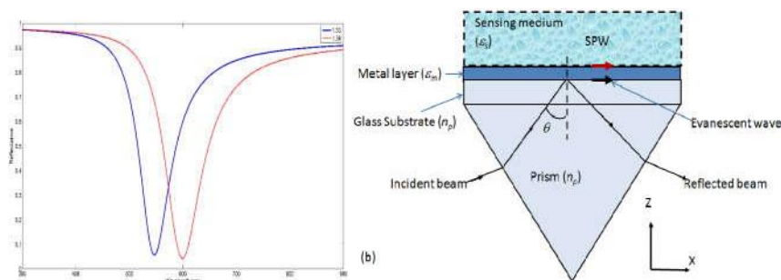
Fig.2(a) Red shift of wavelength and (b) SPR Bioensor
