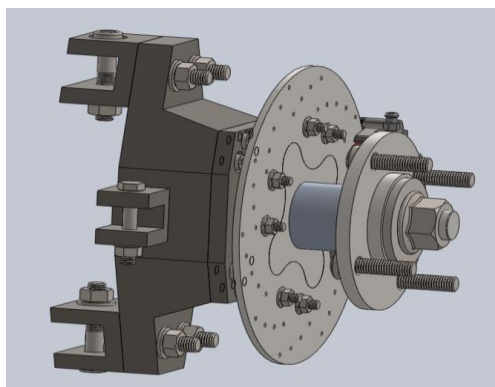
Front upright and hub assembly
