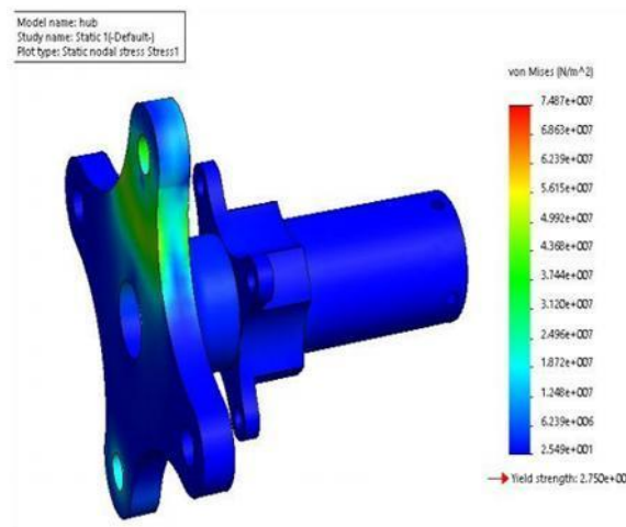
Fig. 5. Design Of Hub as the presented by [12]
