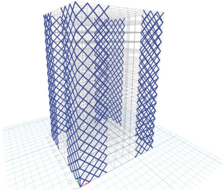
Figure 4: Building with Inverted V Bracing
